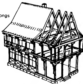
10 In areas short of timber, buildings used wood posts; posts have windows between them and there are braces in the window breasts
